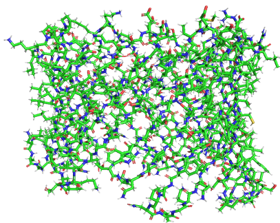
(c) Side view of 3EMN in stick
